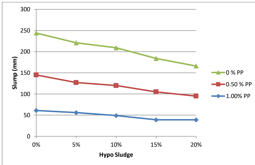
Figure 4: Impact on Slump value of concrete using hypo sludge and polypropylene fiber at various alternate levels of cement
