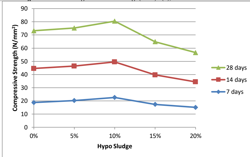
Figure 6: Impact on compressive strength of concrete using 0.50% of polypropylene fiber at various alternate quantity of cement
