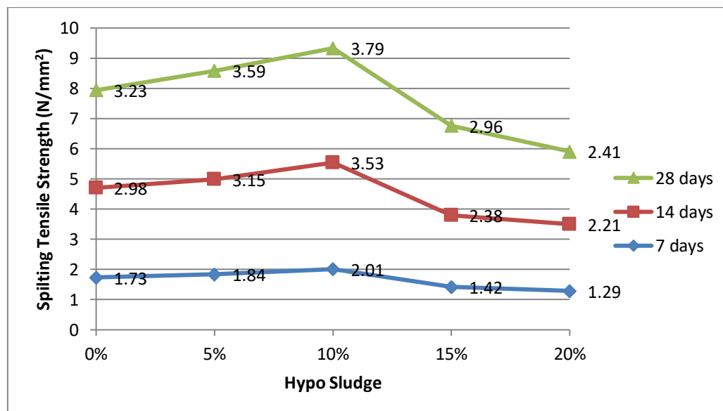
Figure 8: Splitting tensile strength of concrete with 0% addition of PPF at different curing ages
